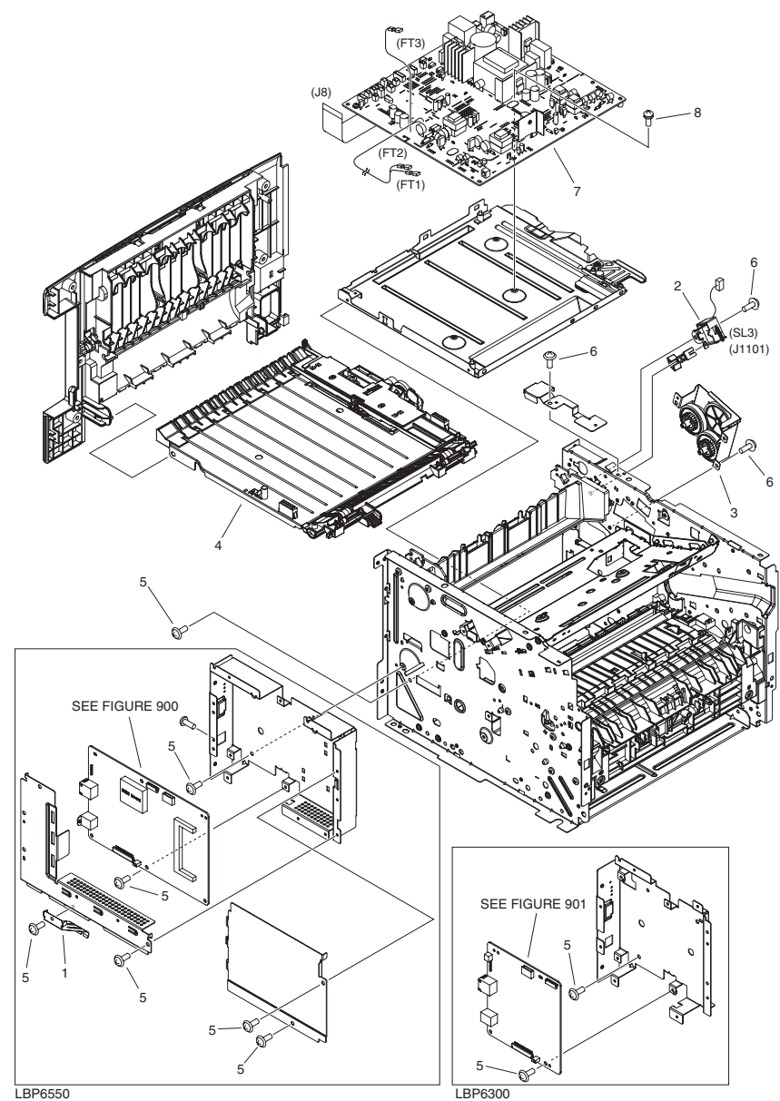
FIGURE 105 INTERNAL COMPONENTS 5
