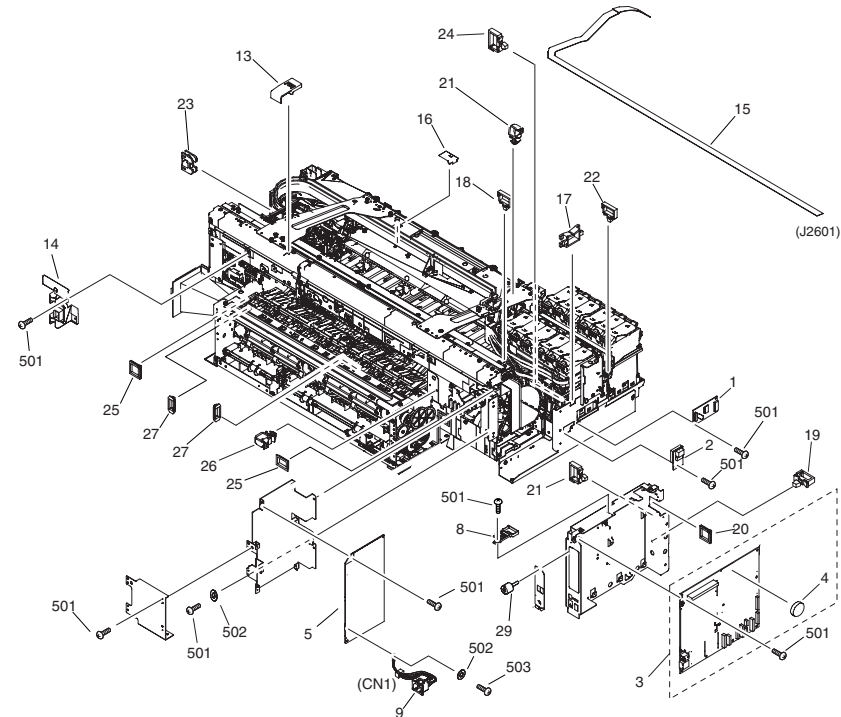
FIGURE 04 ELECTRICAL PART
