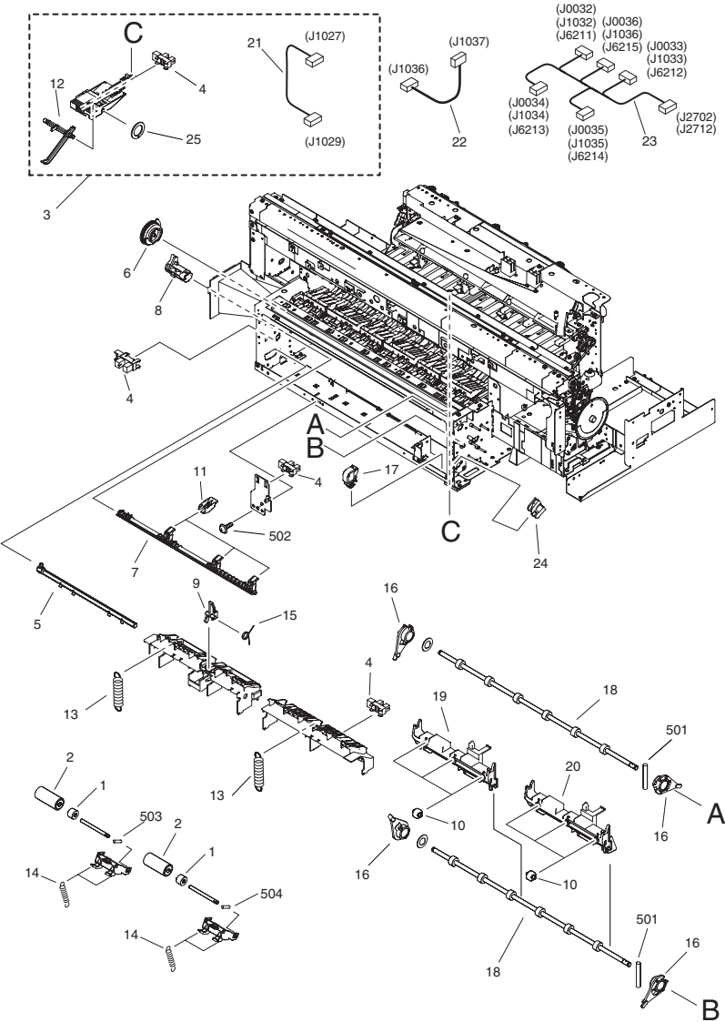
FIGURE 12 PICK-UP & FEED UNIT (2)
