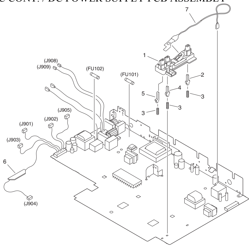
FIGURE 910 DC CONT. / DC POWER SUPPLY PCB ASSEMBLY
