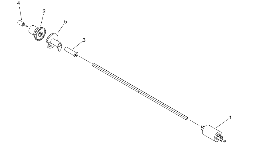
FIGURE 340 PAPER PICK-UP ROLLER ASSEMBLY (MULTI TYPE)
