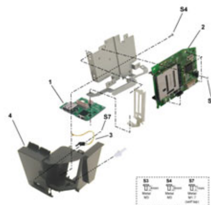
FIGURE 6 FRONT SIDE COVER R UNIT
