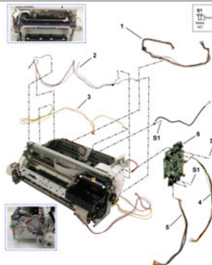
FIGURE 10 CARRIAGE UNIT
