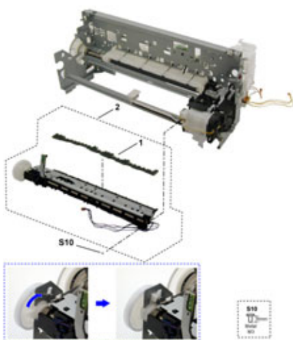
FIGURE 11 PLATEN UNIT
