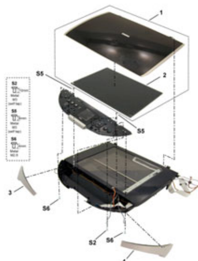
FIGURE 6 FRONT SIDE COVER R UNIT
