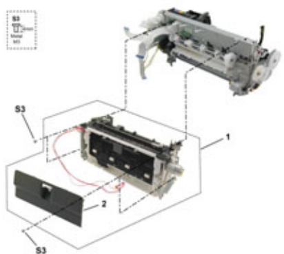
FIGURE 9 SHEET FEED UNIT
