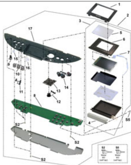
FIGURE 5 OPERATION PANEL UNIT & LCD VIEWER UNIT
