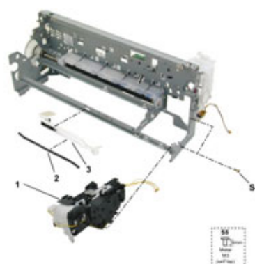
FIGURE 12 PURGE UNIT
