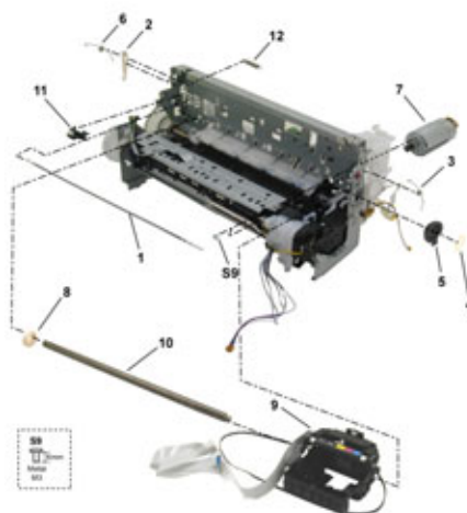
FIGURE 12 PURGE UNIT
